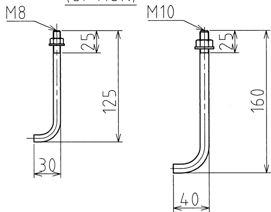
ANCHOR BOLT (OPTION)
