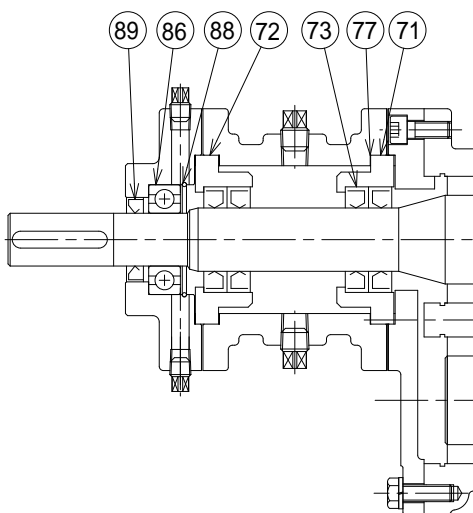
Type: KH-S 2 (OIL SEAL (PTFE))
