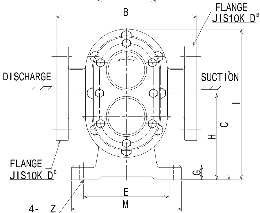
Type: KH-Tv 2 (DOUBLE BELLOWS MECHANICAL SEAL)
